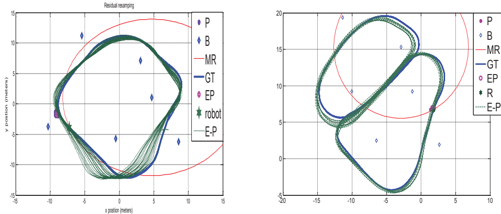
Fig. 6: Residual resampling
