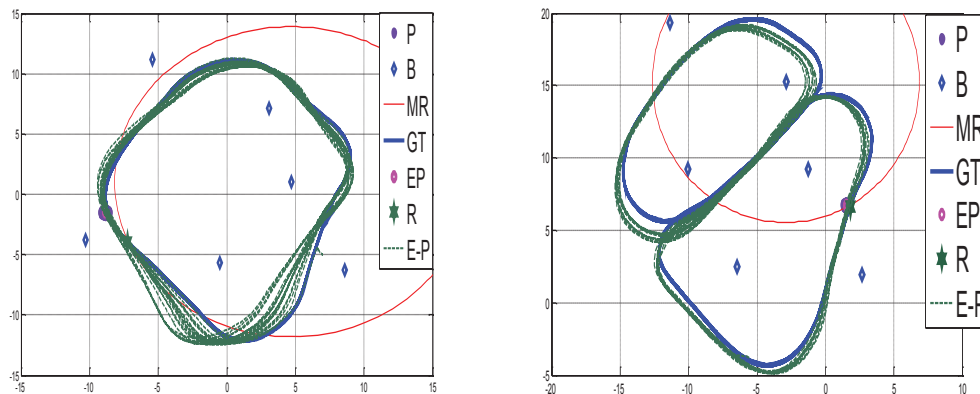
Fig. 5: Multinomial resampling
