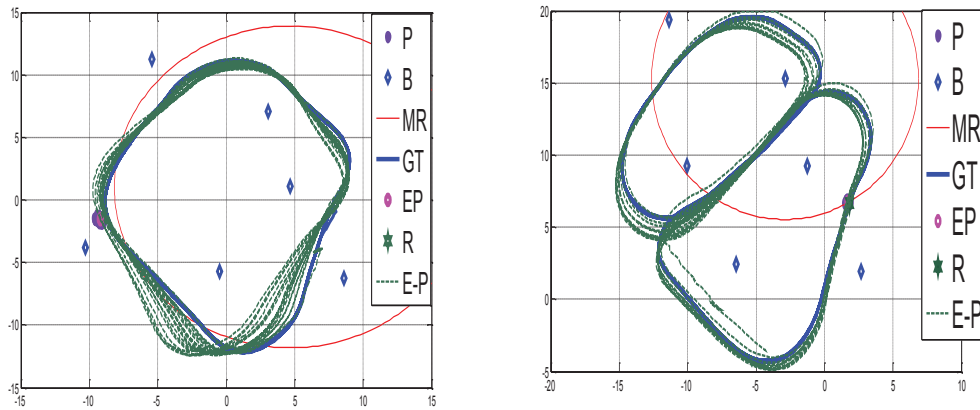
Fig. 4: Stratified resampling
