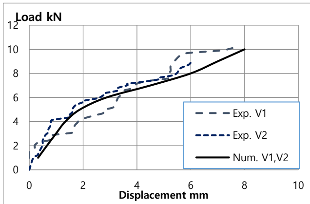
(a) unstrengthened vaults
