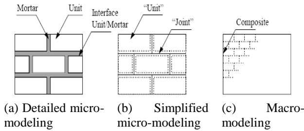
Fig. 1 Modeling strategies for masonry (Lourenco 2002)
