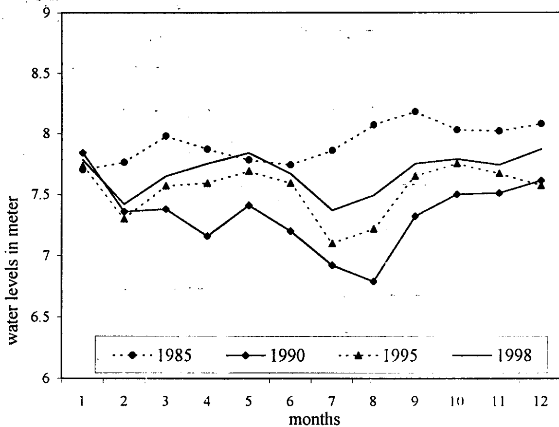
Fig.(21) : Hydrograph showing piezometric head fluctuation of observation well (27) in years 1985, 1990, 1995, 1998.
