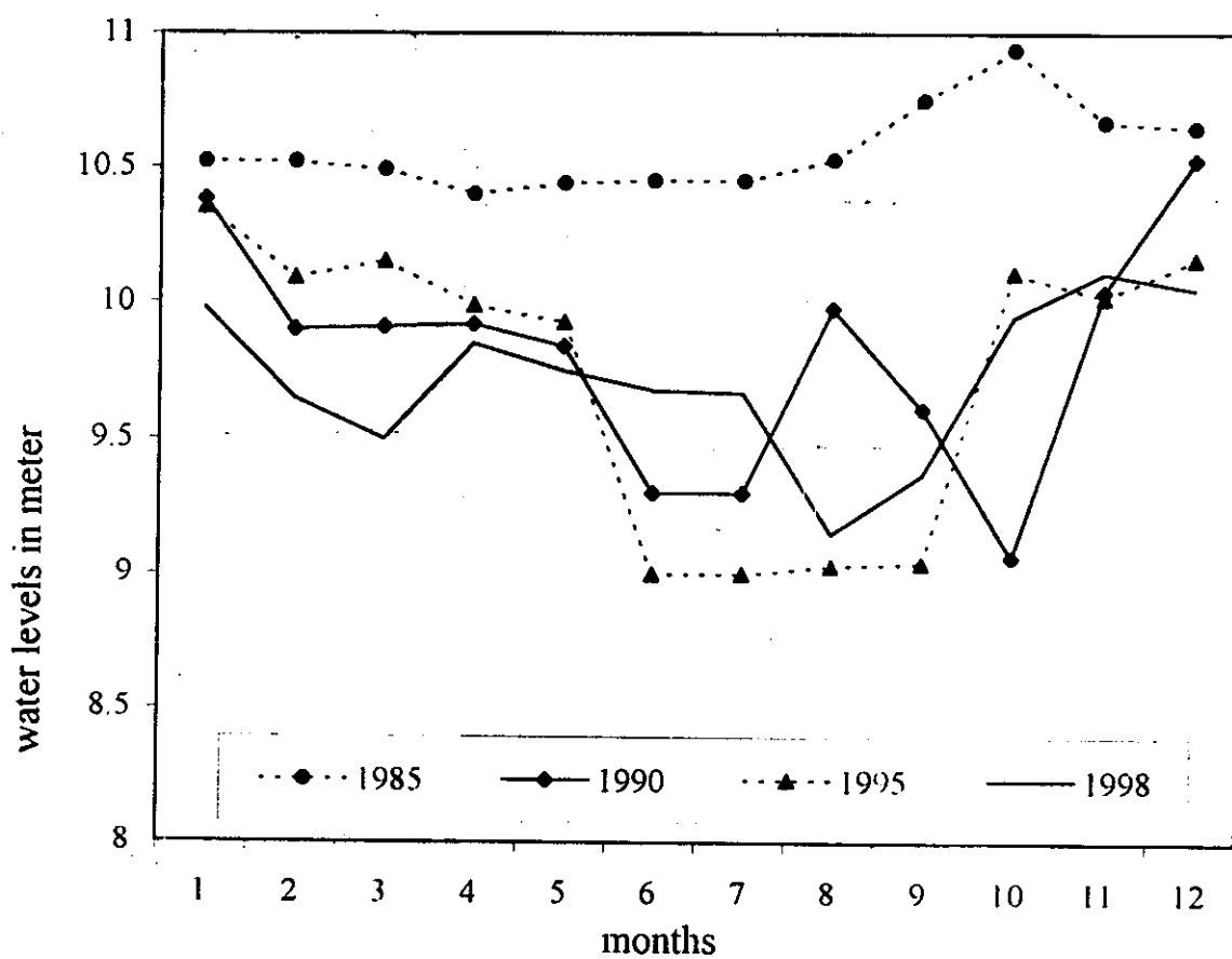
Fig.(22) : Hydrograph showing piezometric head fluctuation of observation well (35) in years 1985, 1990, 1995, 1998
