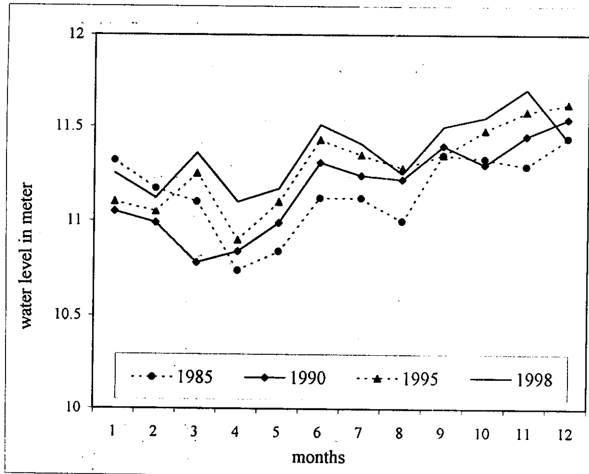
Fig.(24) : Hydrograph showing piezometric head fluctuation of observation well (44) in years 1985, 1990, 1995, 1998.
