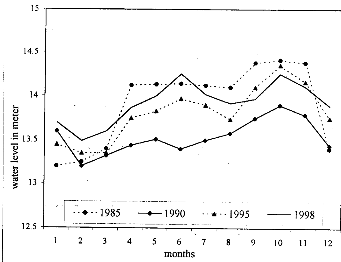
Fig.(23) : Hydrograph showing piezometric head fluctuation of observation well (37) in years 1985, 1990, 1995, 1998.
