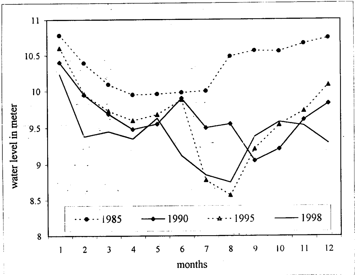
Fig.(25) : Hydrograph showing piezometric head fluctuation of observation well (50) in years 1985, 1990, 1995, 1998.
