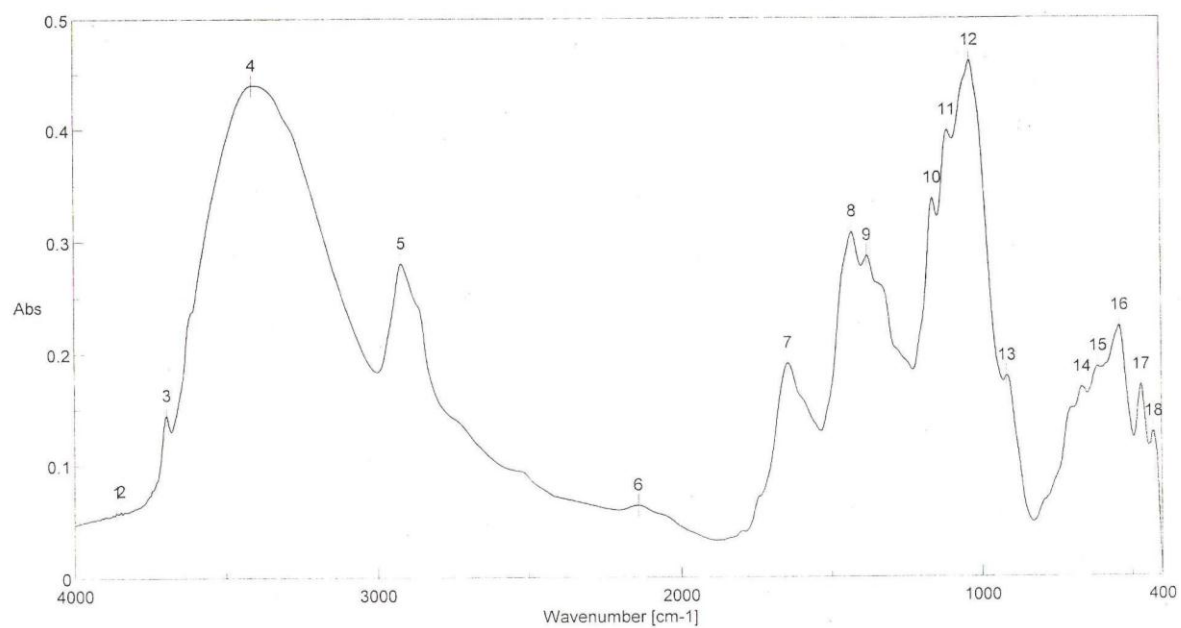
Fig. (G): IR spectra for Quena untreated
