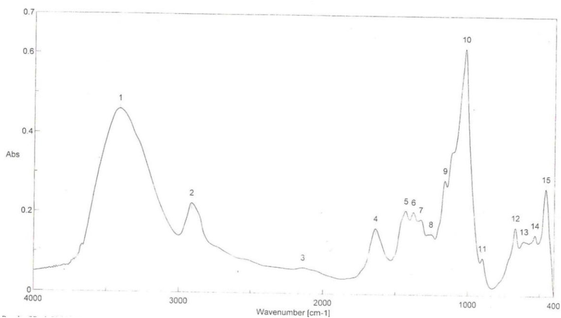
Fig. (F): IR spectra for Edfu treated by borax+ poly (vinyl alcohol). (5% conc.)
