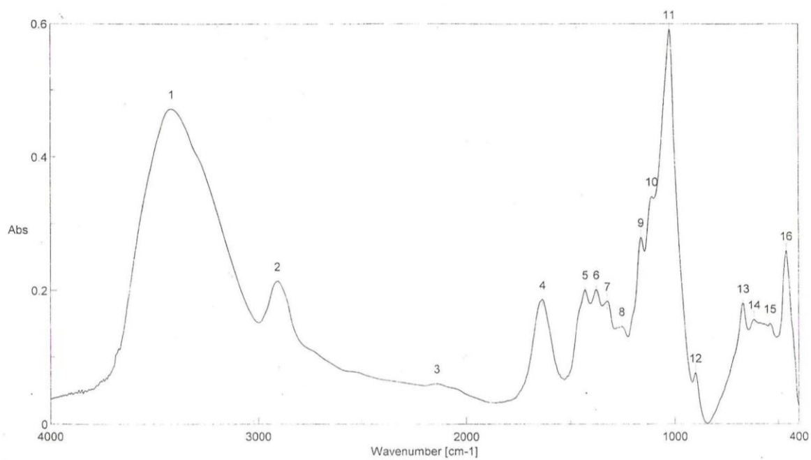
Fig. (B): IR spectra for Edfu treated by ammonium phosphate monobasic (5% conc.)
