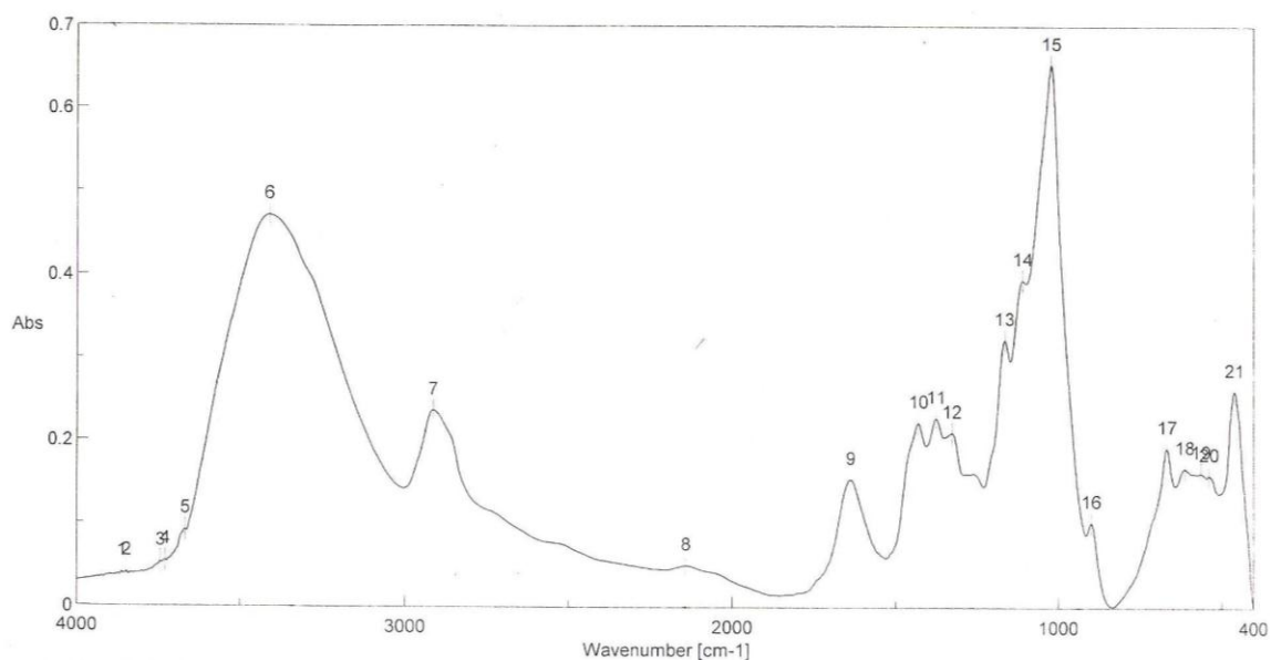
Fig. (D): IR spectra for Edfu treated by borax (5% conc.)
