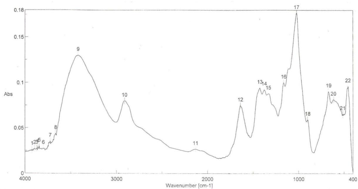
Fig. (E) IR spectra for Edfu treated by boric acid + poly (vinyl alcohol) (5% conc.)
