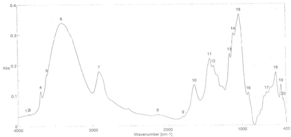
Fig. (H): IR spectra for Quena treated by borax + poly (vinyl alcohol). (5% conc.)
