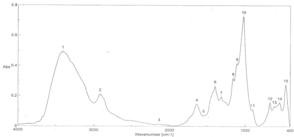
Fig. (A): IR spectra for Edfu untreated
