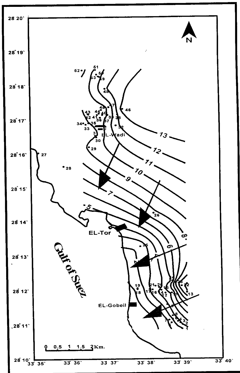
Fig ( 9 ) : groundwater level contour map (m)
