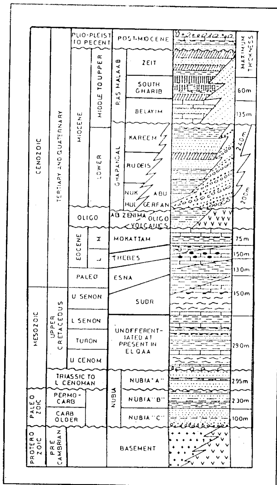
Fig ( 7 ): Stratigraphic sequence of El-Qaa plain
