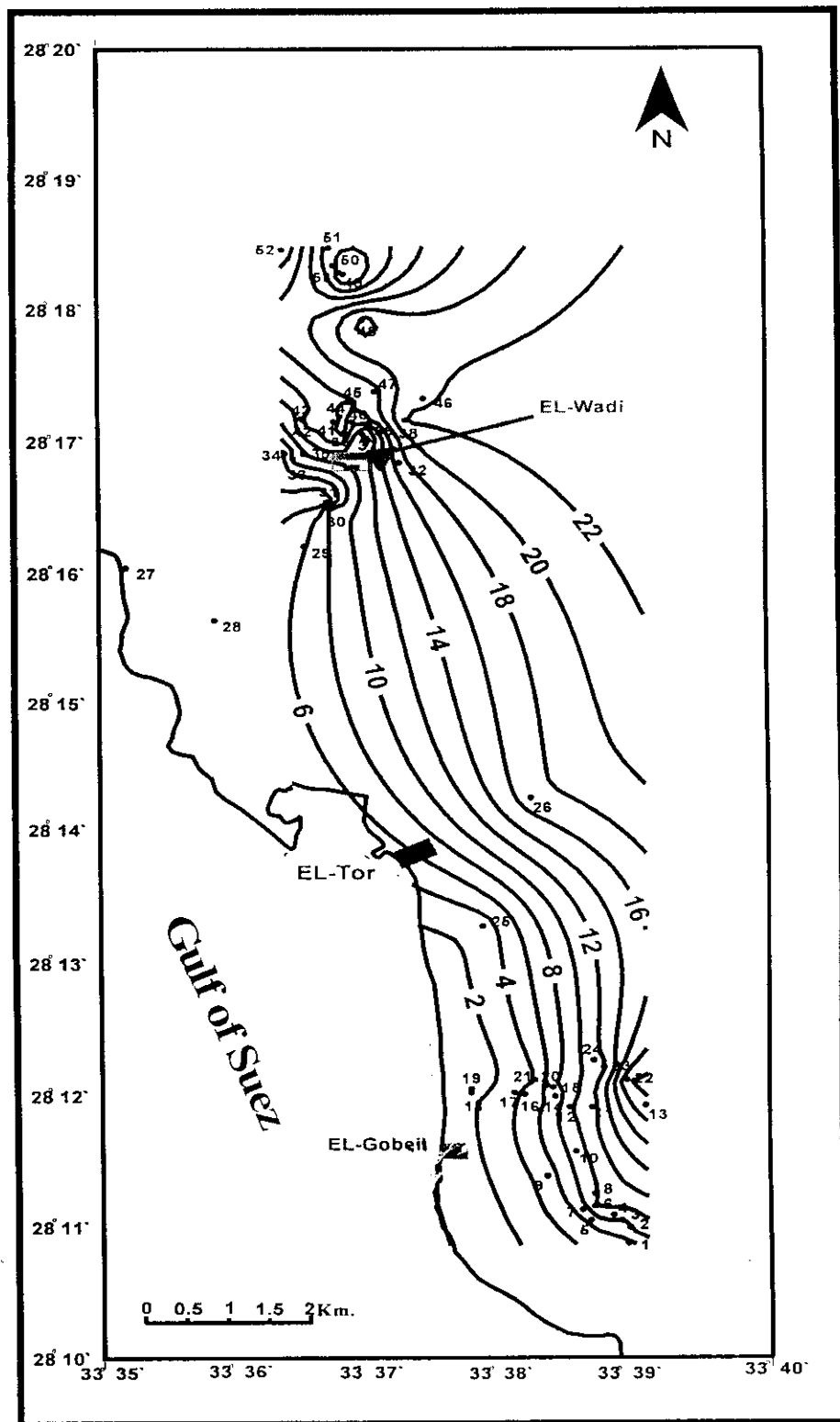
Fig ( 8 ) : Depth to groundwater surface contour map (m)
